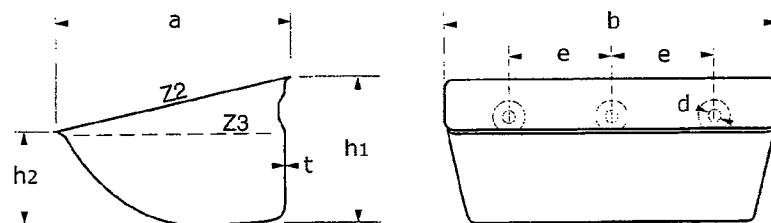
Claus elevator buckets made of steel/stainless steel (parameters in mm)
